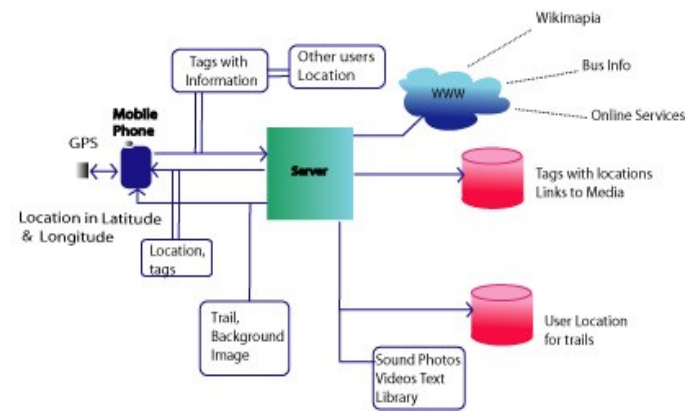
Figure 2: Architecture diagram of WiggleStick
